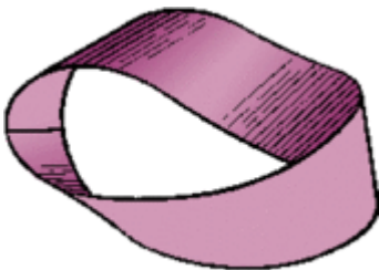
Figure 1 Mobius Strip
